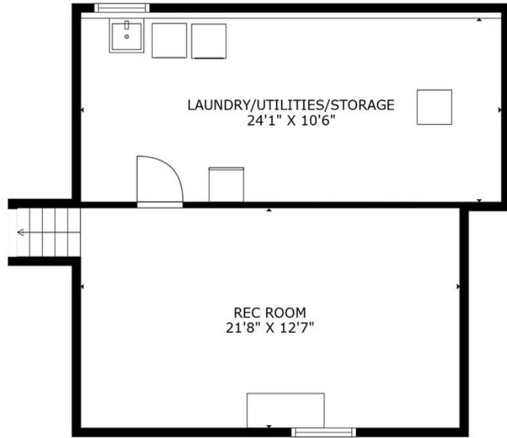
BASEMENT
