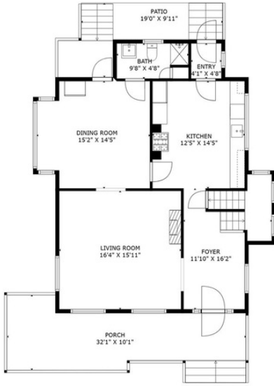
FLOOR 1
